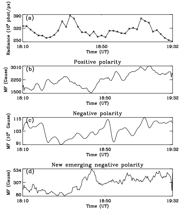
Fig. 2. a) CDS O v 629 Å radiance profile of blinker BL2 obtained by integrating over the blinker area; b) temporal evolution of the total magnetic flux (MF) from positive polarity fragments above 40 Gauss associated with BL2; c) total magnetic flux from negative polarity fragments above 40 Gauss underlying the loop associated with BL2; d) temporal variations of the new emerging magnetic flux of negative polarity above 15 Gauss appearing in the BL2 position.
