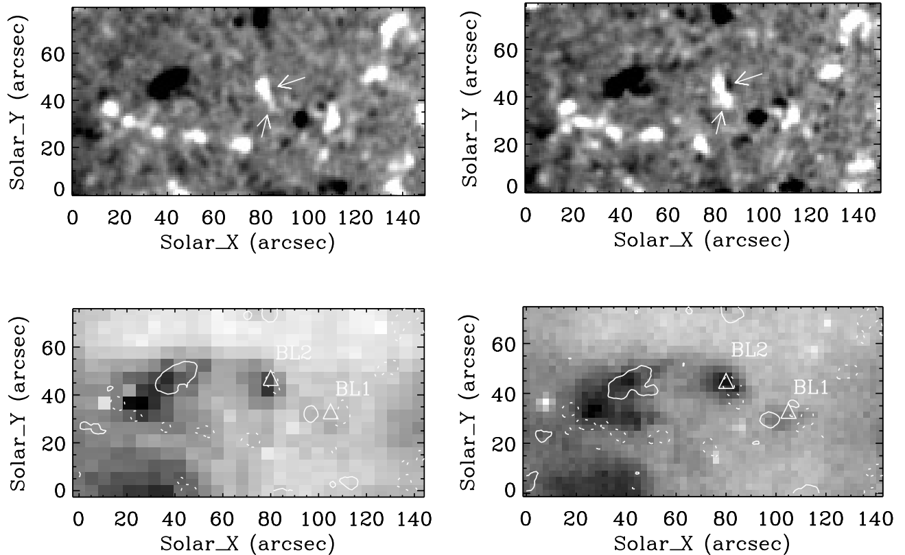
Fig. 1. BBSO magnetograms ( top row ) with simultaneous reversed colour EIT Fe XII 195 Å images ( bottom row ), with the left two panels taken at 18:24 UT, and the right panels at 19:13 UT on October 23, 2001. BL1 and BL2 indicate the blinkers positions. The contours overlotted on the EIT images represent the \pm 25 G negative (solid line) and positive (dashed line) magnetic flux. The arrows point towards the newly emerging magnetic fluxes while the triangles show the locations of the blinkers identified in the CDS data. In Madjarska & Doyle (2003), these blinkers were labelled BL1 and BL2.
